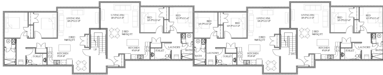
2 SECOND-FOURTH FLOOR UP-11' 508 SQ FT
