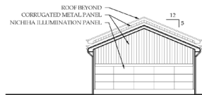
C2 GARAGE ELEVATIONS 12'-0"
