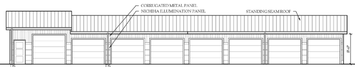
C3 GARAGE ELEVATIONS 8'-0"
